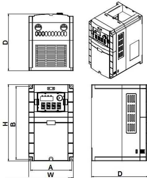
FigureD-1 Frequency converter 0.75KW~315KW external dimension
